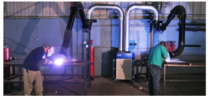
The powerful fan and cleanable filter media in the Model 500/550 Dual Stand Assembly can help protect two workers from welding fumes for heavy-loading applications.
